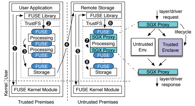
Fig. 1: TRUSTFS' architecture.
