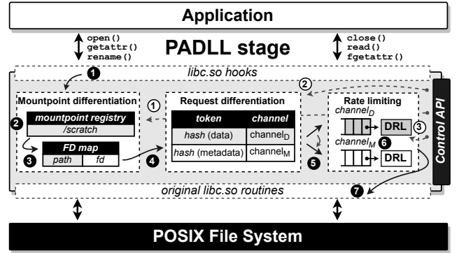
Fig. 5: PADLL data plane stage design and operation flow. Black circles depict the operation flow of intercepted POSIX requests, while white circles depict housekeeping and control operations of PADLL.
