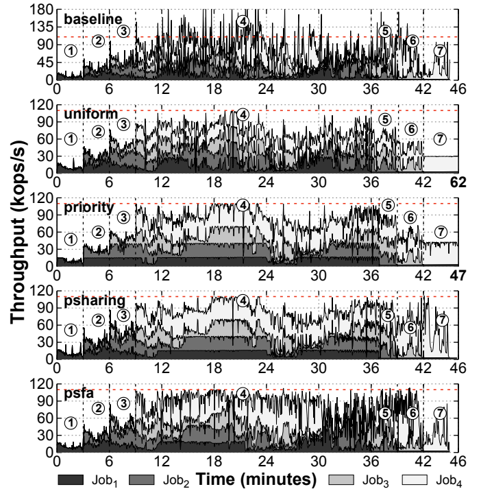
Fig. 8: Per-job metadata control over Baseline, Uniform, Priority, PSharing, and PSFA setups under testing scenario #2.
